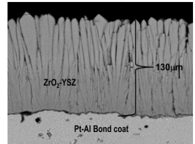
Typical microstructure of ZrO 2 -YSZ coatings
