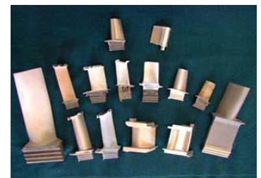
TBC coated blades for aero engine
